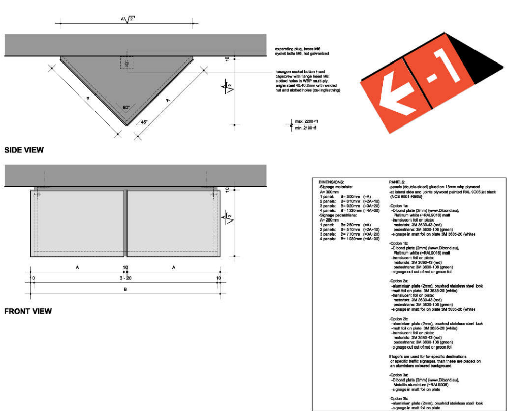
Figure 59: Signage angled from the ceiling
