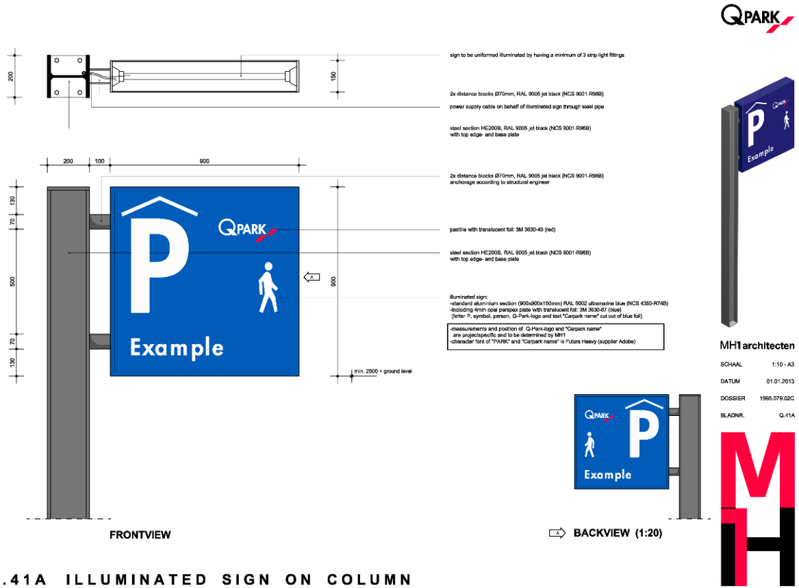
Figure 62: Illuminated P-sign for pedestrians on column
