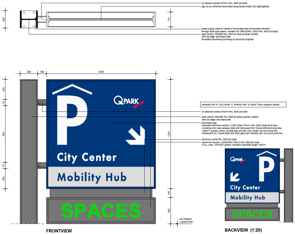
MQ01B.1 Illuminated sign on column - Mobility Hub
