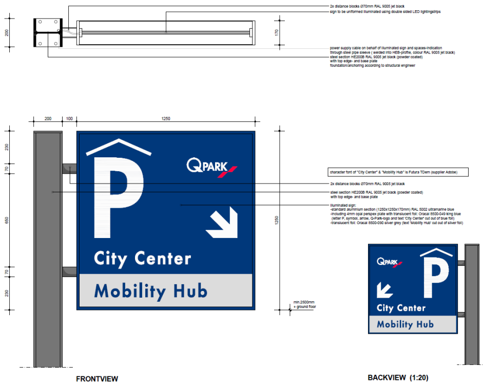
MQ01B.2 Illuminated sign on column - Mobility Hub
